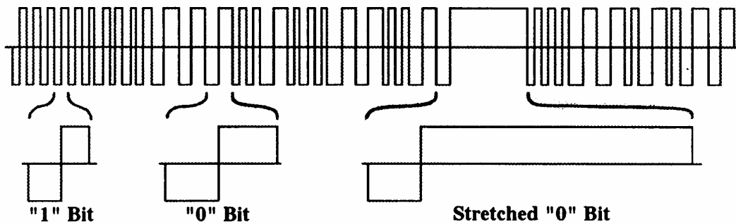
25 Figure 1: Bit Encoding
